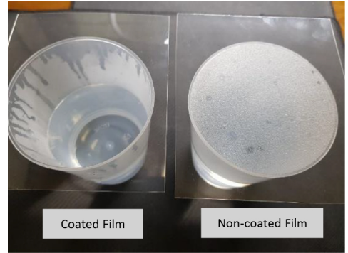
Steam Test - 80°C Hot water
